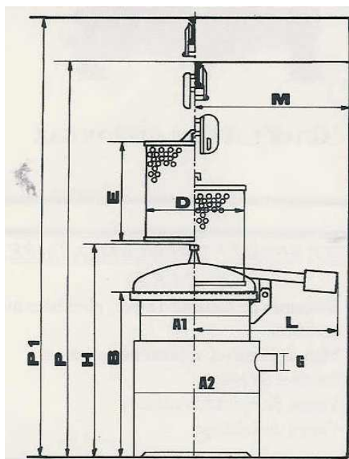
Autoclave Gaz
